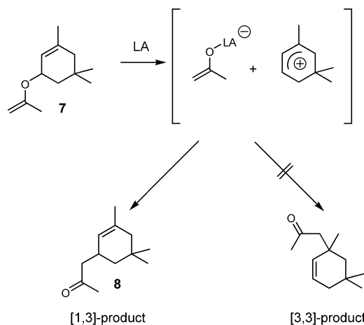
Figure 2. Ionic pathway for the synthesis of [1,3]-Claisen products.
