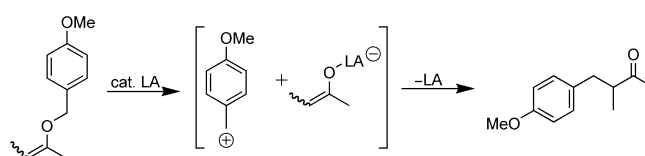
Figure 1. Concept for the Lewis acid-catalyzed alkylation of enolates.
