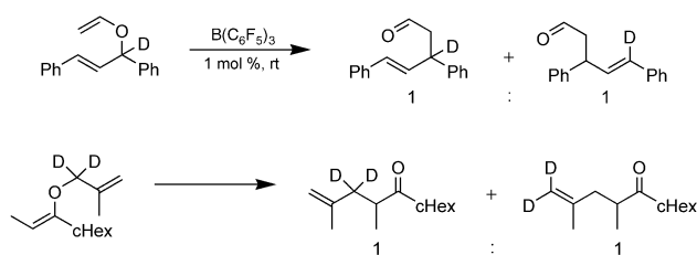
Figure 3. Deuterium labeling studies as proof of a non-concerted mechanism.
