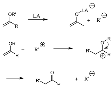
Figure 4. Addition to enol ethers via a chain mechanism as alternative to enolate alkylation.
